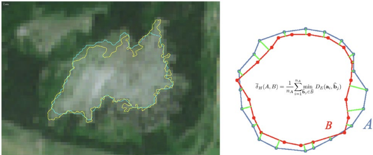
A6_Fig 3 Example of gps track (yellow) and automatic segmentation (blue) and the formula of Hausdorff distance used for comparison of two curves
