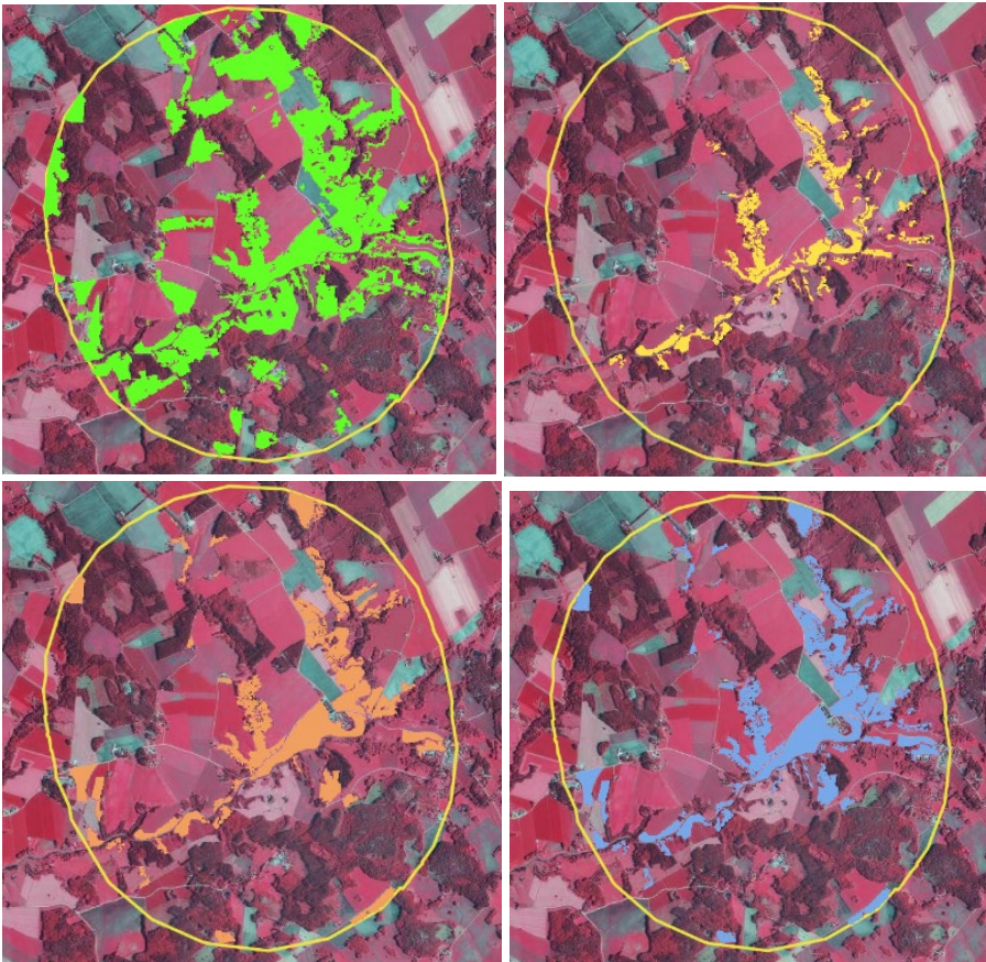
A4_Fig 10 Examples of the grassland product in Rekijokilaakso, a Natura 2000 -site (green), and the three reference grassland masks and they polygons shown as different colours: SAKTI mesic grasslands (yellow), LPIS open grassland habitats (orange) and combined SAKTI+LPIS (blue).
