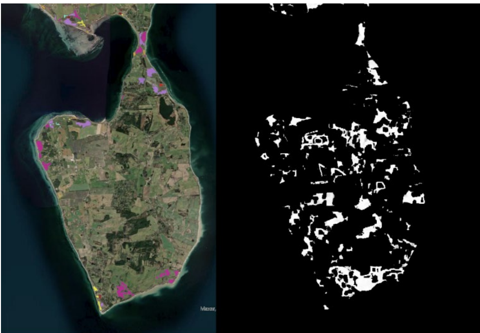
A6_Fig 14 . Relevancy map for the habitat complex 6230/6210
